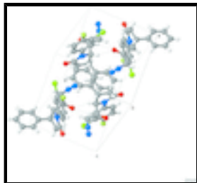
Fig. 2. Part of the crystal structure showing carbonyl oxygen O2 interacts with three H atoms.
